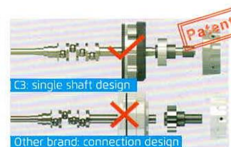
Single shaft drive; Stable and fast
